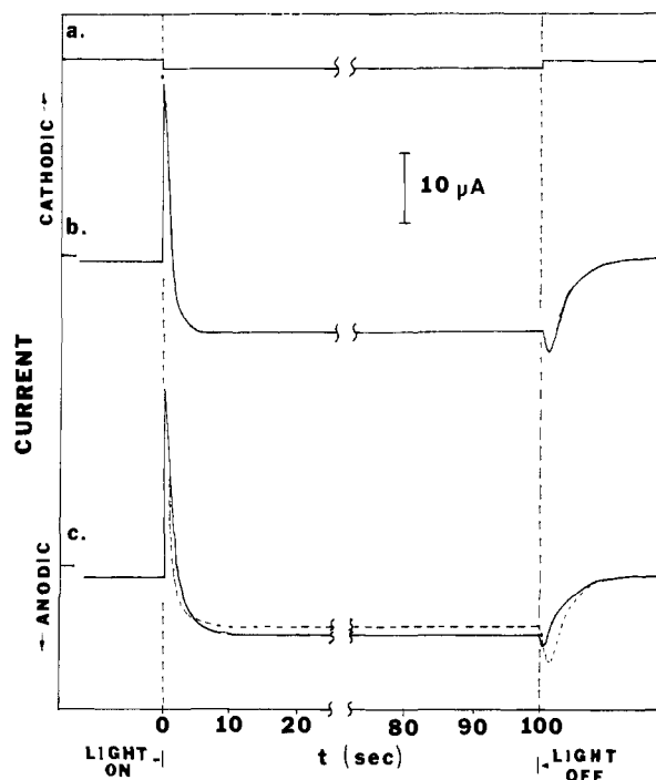
Figure 4. Photocurrent response in 0.02 M HCl of (a) Pt electrode, (b) \text{TiO}_2 slurry at Pt electrode, (c) \text{TiO}_2 slurry at Pt electrode in two-electrode cell (Figure 5); (---) stirred, (—) unstirred.
